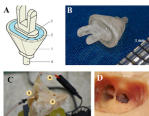
Fig.1-The ChSP prototype (A,B) and experimental setup (C,D). B-temporal bone, S-speaker, M-microphone
