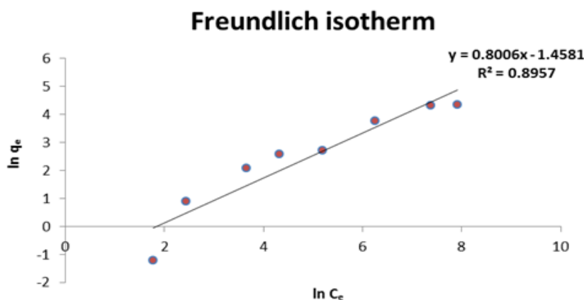
Figure 11: Linear freundlich isotherm.
