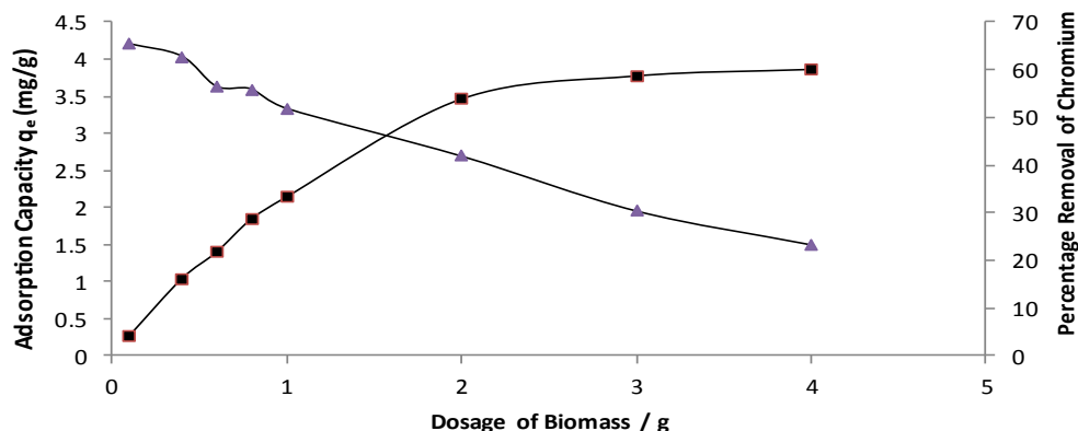
Figure 2: Percentage removal of the total chromium from leather tannery effluent and adsorption capacity at different biosorbent dosage of Cabomba caroliniana [Concentration of effluent-1470 ppm, Optimized pH-4.5, Contact time-3 h, Agitation speed-100 rpm, Room temperature-30°C].
