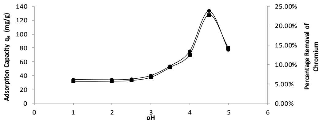
Figure 1: Percentage removal of the total chromium from leather tannery effluent and adsorption capacity of biosorbent at different pH by Cabomba caroliniana [Raw effluent (~6000 ppm) - Biosorption dosage-1.000 g, Contact time-3 h, Agitation speed-100 rpm, Room temperature-30.1°C].
