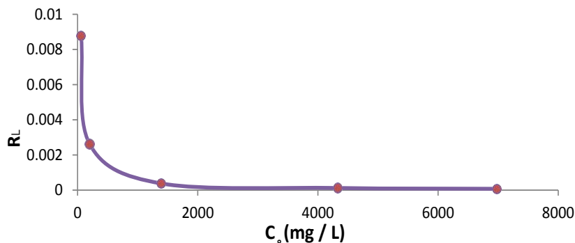
Figure 10: R_L versus initial concentration.
