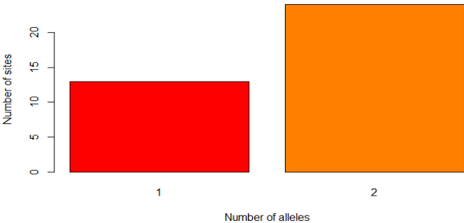
Figure 4: Distribution of the number of alleles per loci of dhfr genes.
