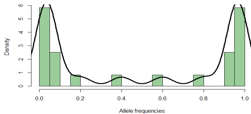
Figure 7: Distribution of alleles frequencies of dhps genes.
