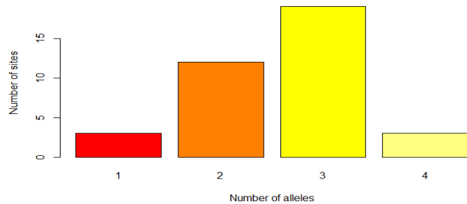
Figure 5: Distribution of the number of alleles per loci of dhps genes.
