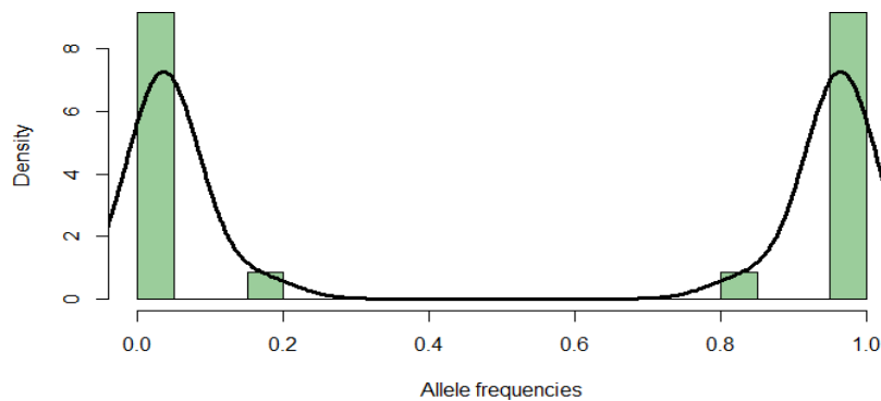
Figure 6: Distribution of alleles frequencies of dhfr genes.
