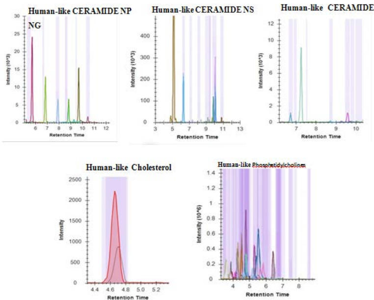
Figure 2: Chromatogram images of Human-like ceramides, Cholesterol and PC in Nannochloropsis gaditana extract obtained by High Performance Liquid Chromatography/ Mass Spectrometry (HPLC/MS).
