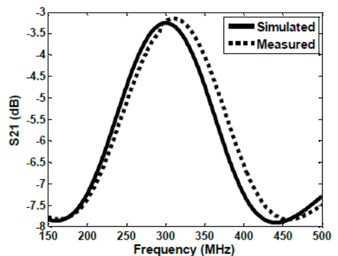
Figure 3: Simulation and measurement-insertion loss, S_{21} -(dB).
