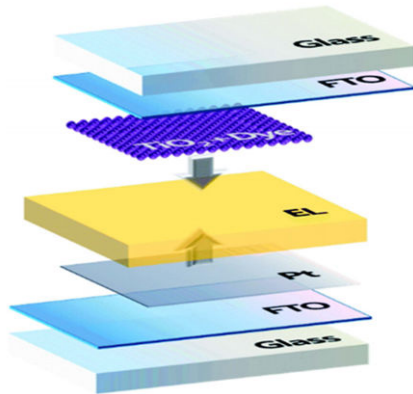
Figure 1: Components of dye sensitized solar cells.
