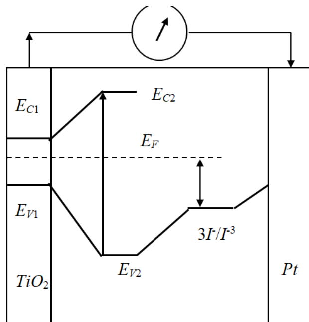
Figure 3: Zone diagram of the DSSC solar cell.
