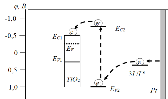
Figure 2: \text{TiO}_2 -based DSSC solar cell operating principle. EC1-and EV1 are the boundaries of the conductivity and valence band of \text{TiO}_2 , respectively, EC2-and EV2 are the boundaries of the conductivity and valence band of the dye, EF-Fermi level.
