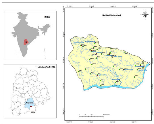
Figure 1: Location map of Nellikal watershed of Nalgonda district, Telangana along with sampling stations.
