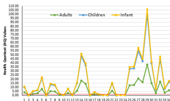
Figure 7: Scatter plot showing HQ > 1 for nitrate concentration in all groundwater samples indicating children.
