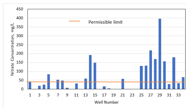
Figure 6: Nitrate levels in the groundwater of Nellikal watershed.
