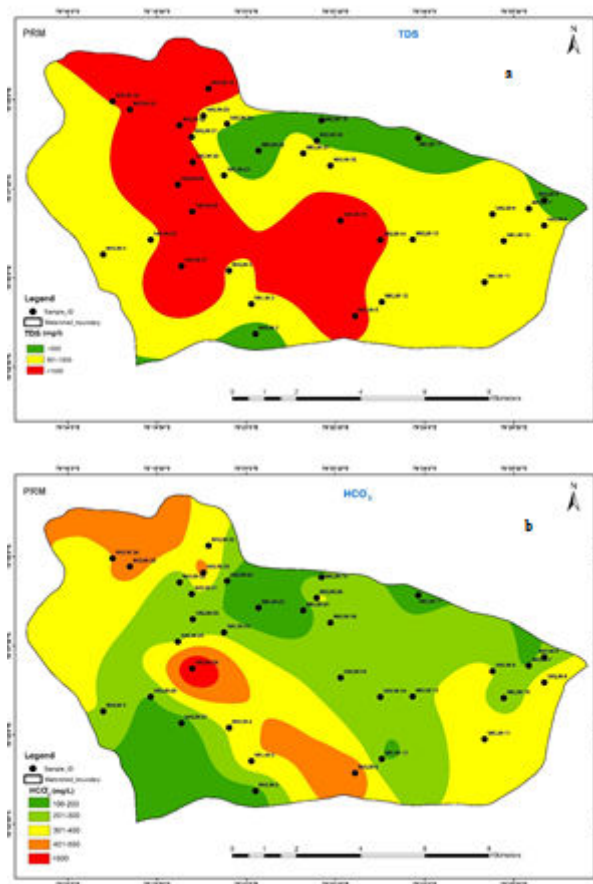
Figure 2: Spatial distribution maps of (a) TDS, (b) Bicarbonate.
