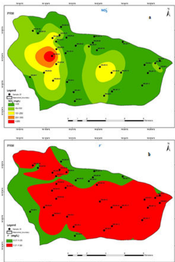
Figure 3: Spatial distribution maps of (a) Nitrate (b) fluoride in groundwater.
