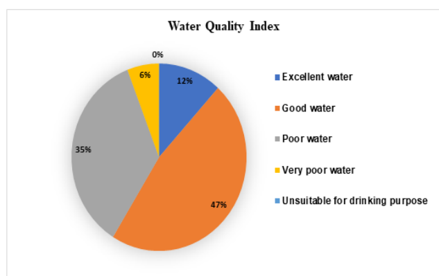
Figure 5: Distribution of percentage of WQI values of groundwater in the study area.
