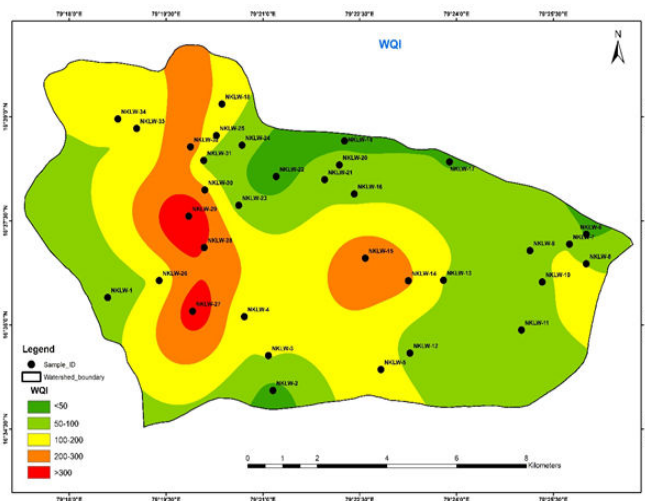
Figure 4: Spatial variations of WQI values of groundwater in the Nellikal watershed.
