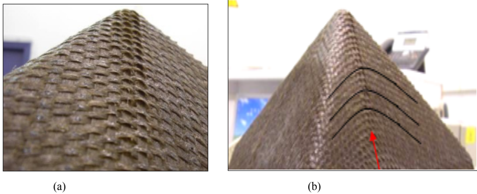
Figure 3: (a) Buckling on face (b) Rovings' orientation.
