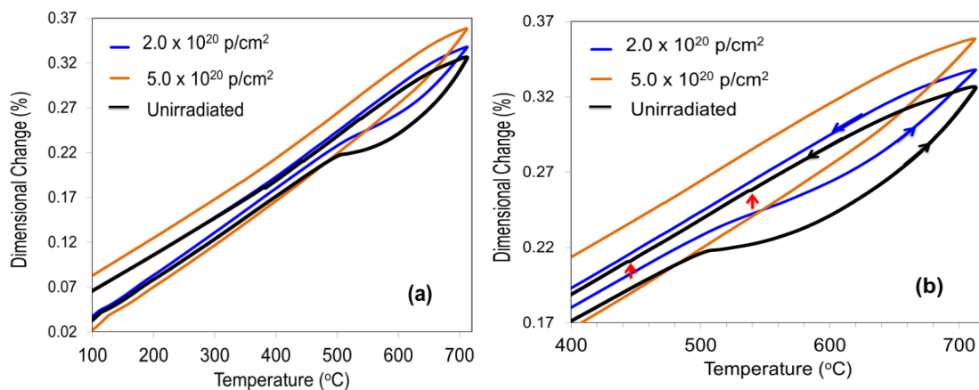
Figure 5: Dimensional stability of the 50% CW Mo during the first post-irradiation thermal cycle.
