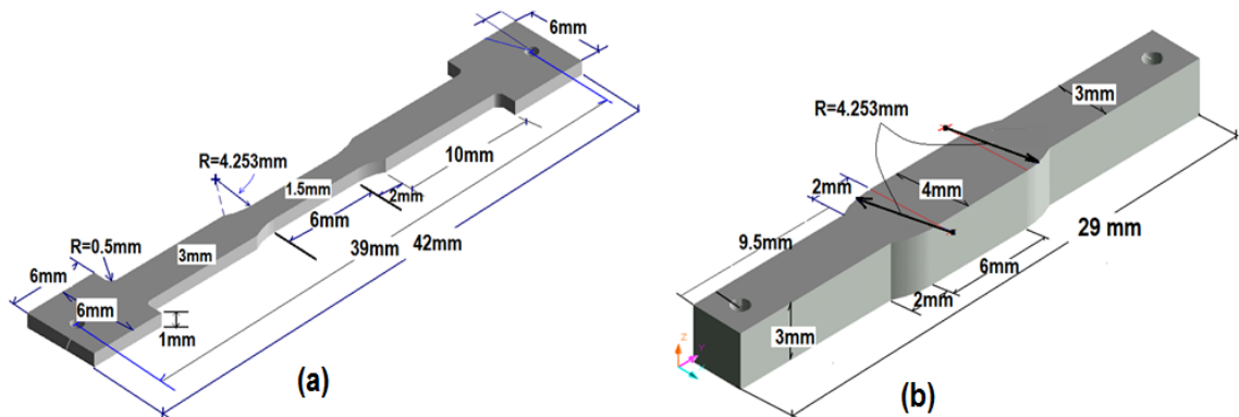
Figure 2: Geometries of irradiated Mo specimens. (a) Tensile sample and (b) CTE-type sample.
