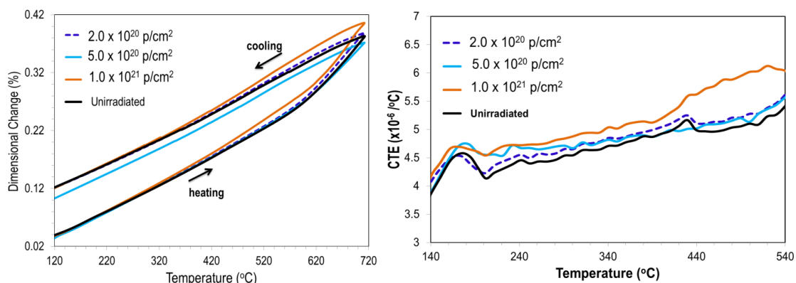
Figure 6: (a) Post-irradiation annealing (2 nd thermal cycle) of irradiated Mo and, (b) thermal expansion coefficient as a function of temperature and dose.
