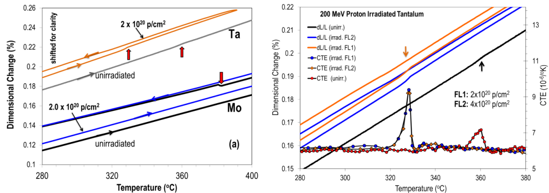
Figure 7: (a) Dimensional change comparison with irradiated Ta to same fluency, and (b) Ta magnetostriction "anomaly" in dimensional change and CTE in the temperature window 320-360°C.
