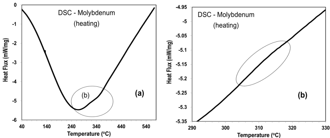
Figure 3: DSC analysis of the 50% CW Mo. Shown in (b) is the presence of a "transition" near 320°C.
