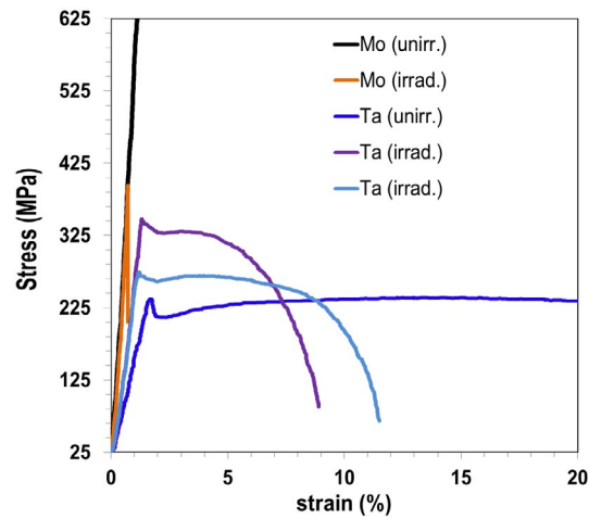
Figure 9: Comparison of the irradiated 50% CW Mo with irradiated Ta.
