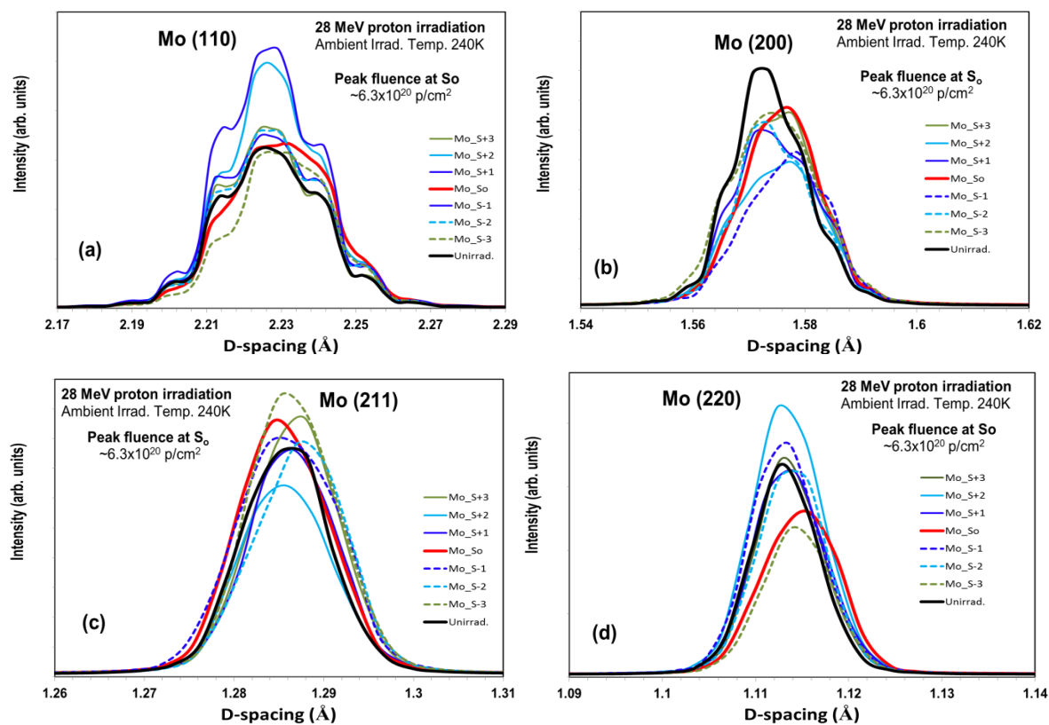
Figure 13: Crystal plane reflection comparison between as-received and proton-irradiated Mo.
