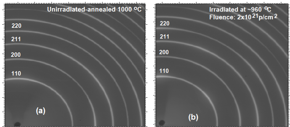
Figure 14: Diffraction pattern comparison between as-received and proton-irradiation Mo.
