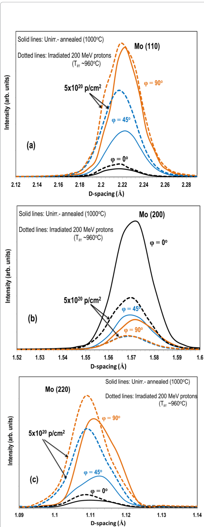
Figure 15: Proton irradiation effects on the microstructure of Mo.
