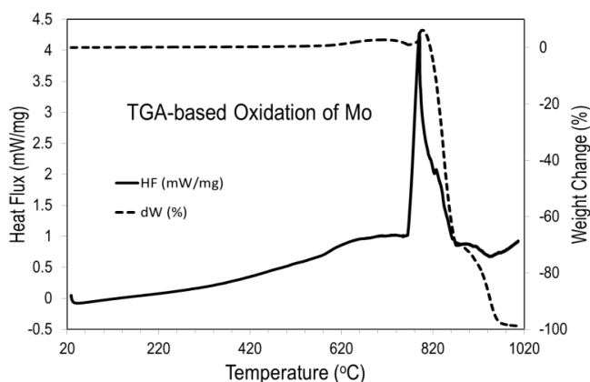
Figure 4: TGA-based oxidation behavior of the 50% CW Mo.
