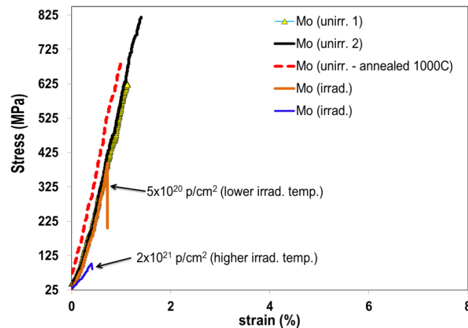
Figure 8: Stress-strain behavior of 50% CW Mo as a function of proton fluency and annealing.
