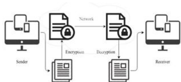
Figure 3: Simple cryptography.
