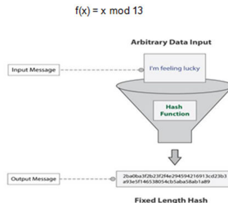
Figure 6: Mechanism of hash function.
