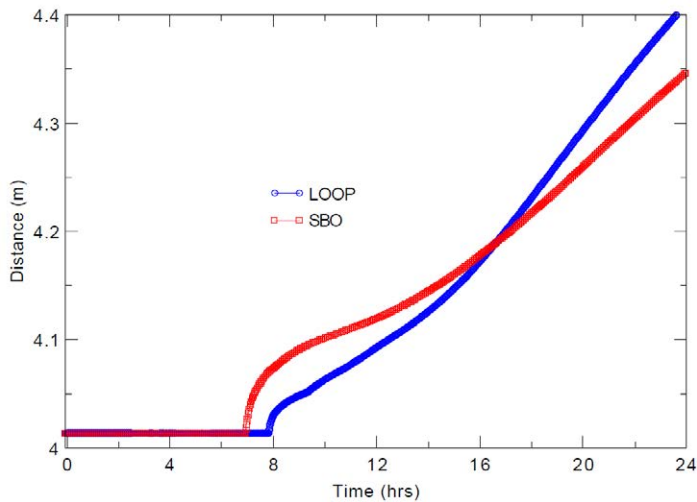
Figure 10: Radial coordinate of core catcher body for SBO and LOOP condition.
