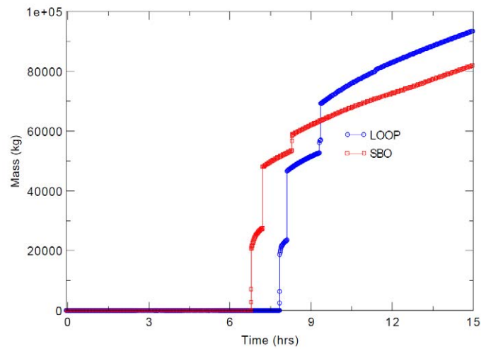
Figure 7: Total mass of Heavy mixture in core catcher in SBO and LOOP condition.
