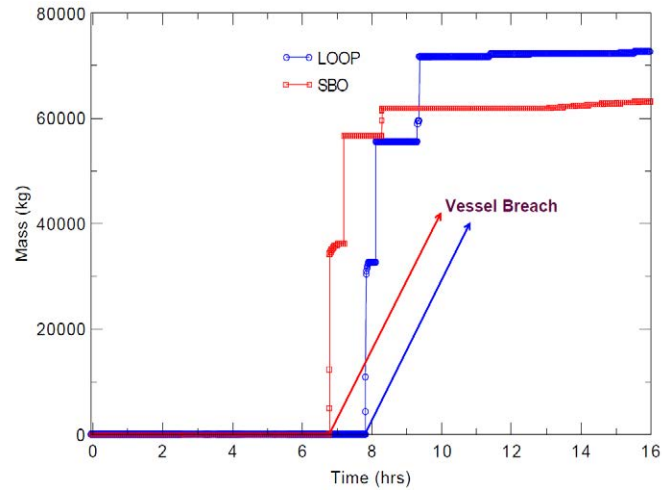
Figure 6: Core melt ejection through vessel breach in SBO and LOOP condition.
