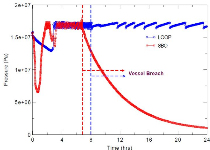
Figure 5: Reactor coolant pressure for SBO and LOOP accident.
