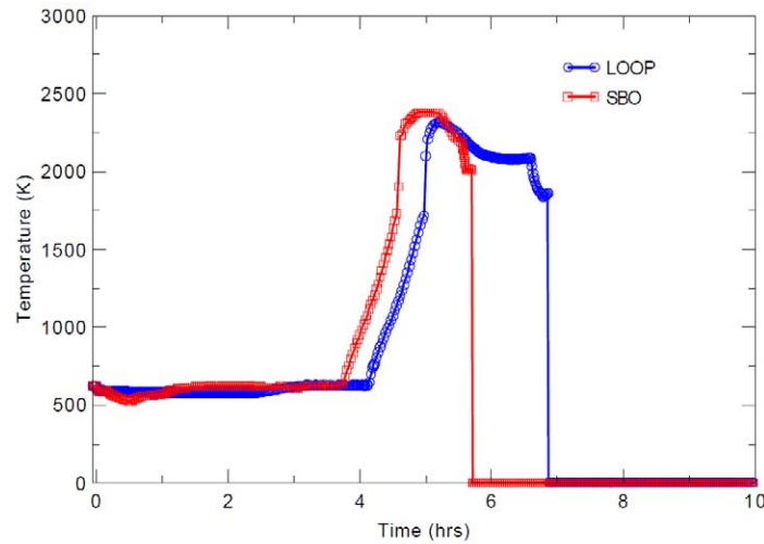
Figure 4: Peak clad temperature for SBO and LOOP accident.
