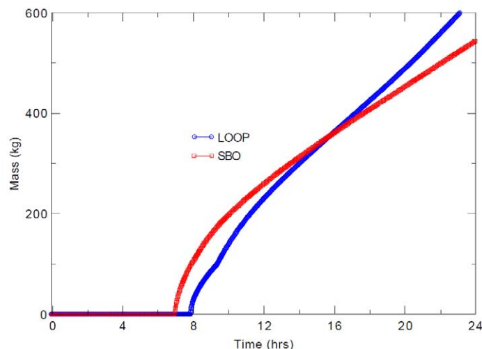
Figure 12: Total CO production from MCCI in core catcher for SBO and LOOP condition.
