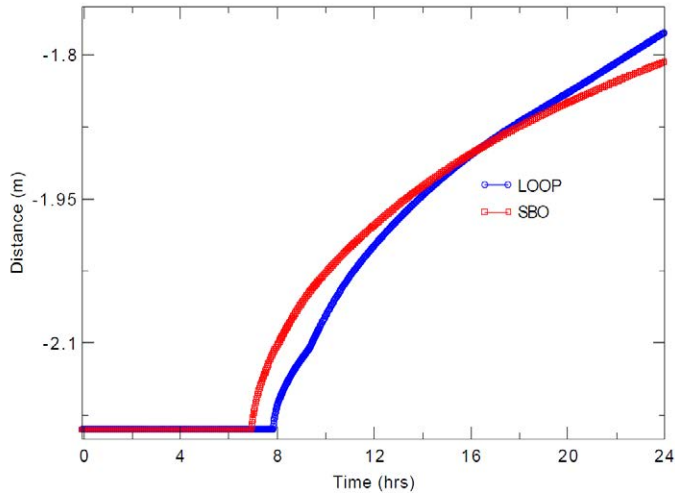
Figure 9: Axial coordinate of core catcher body for SBO and LOOP condition.
