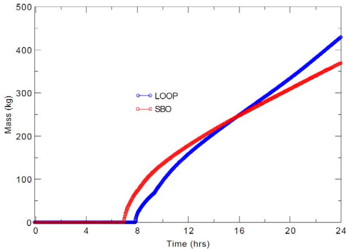
Figure 11: Total H 2 production from MCC1 in core catcher for SBO and LOOP condition.
