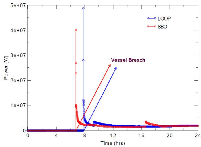
Figure 8: Heat loss to concrete for SBO and LOOP condition.
